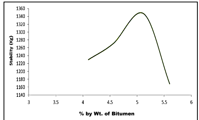
Fig. 1: Effect of Binder Weight on Stability
